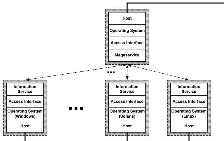
Figure 1: Composing Autonomous Services Into Megaservices
