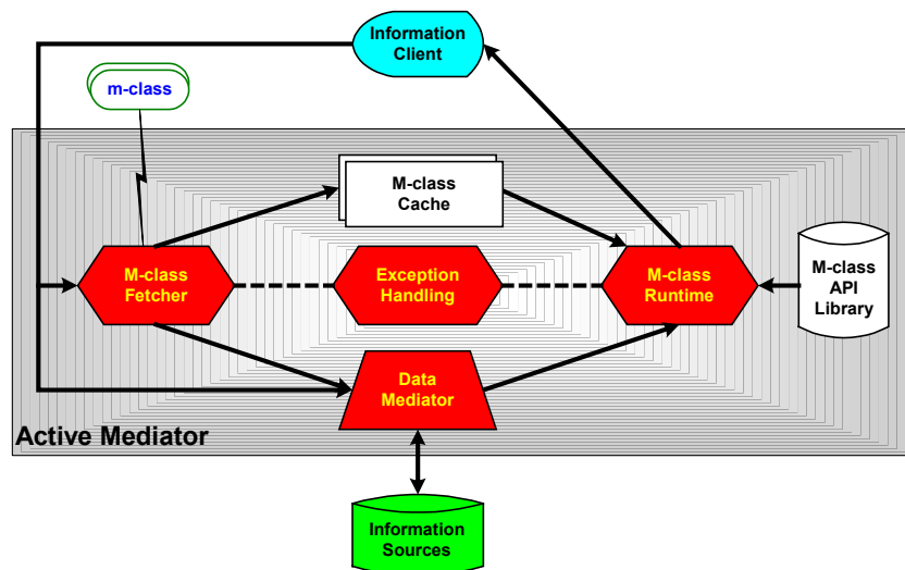
Figure 3: Active Mediation Architecture
