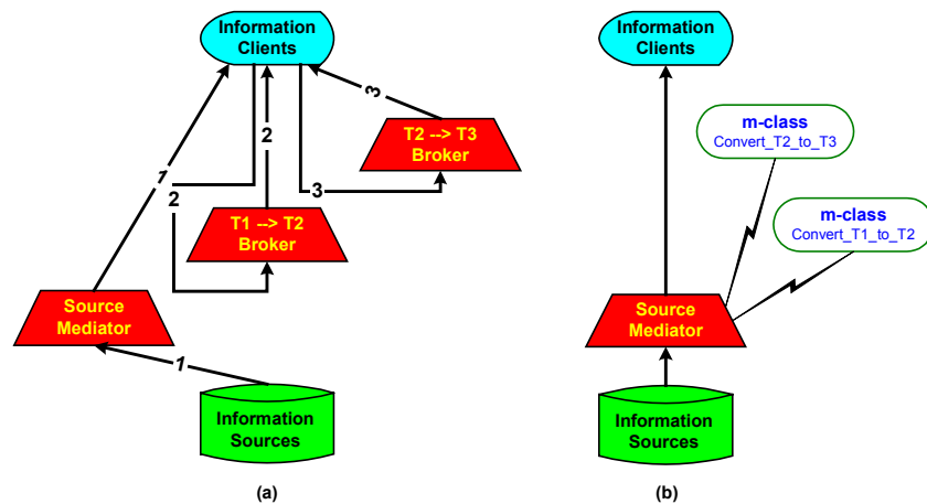
Figure 5: Type Conversion for Autonomous Services
