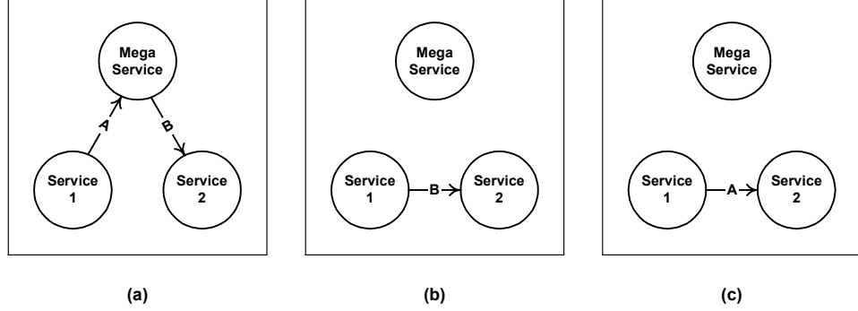
Figure 8: Data-flow Diagrams for the Sample Megaservice using M-class Sum
