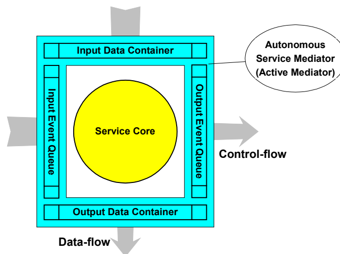
Figure 4: Autonomous Service Metamodel
