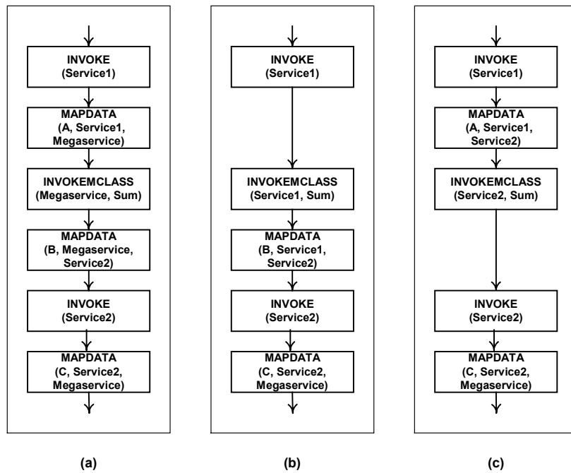
Figure 7: Execution Plans for the Sample Megaservice using M-class Sum
