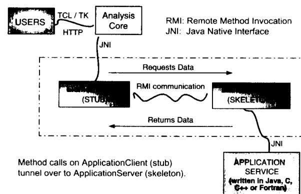
Fig. 8. Mechanics of the distributed element service.
