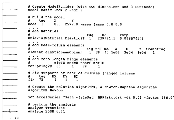
Fig. 13. The model and part of the input Tcl file.
