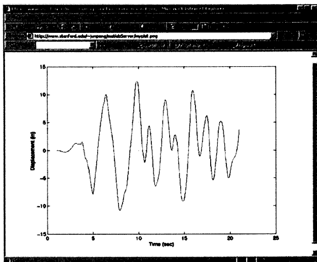
Fig. 15. Graphical response time history of Node 1.
