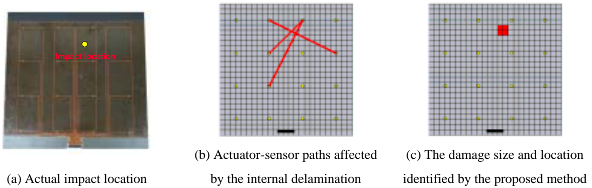
Figure 9: Detection of different sizes of damage using the wavelet-based approach
