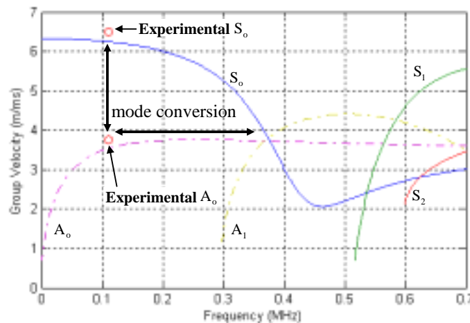
Figure 2: A dispersion curve for an idealized isotropic composite plate
