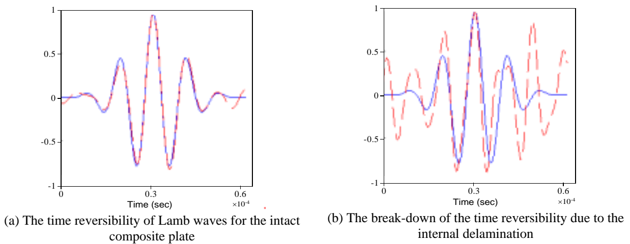
Figure 10: Comparison between the original input signal (solid) and the restored signal (dotted) during the TRA process between actuating PZT # 6 and sending PZT #9
