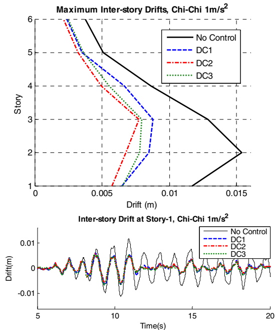
Fig. 4: Experimental Interstory Drift Results
