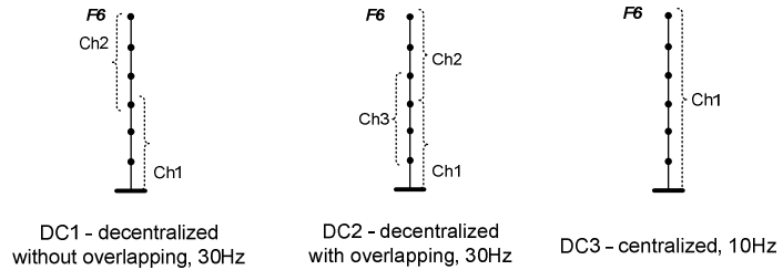
Fig. 3: Experimental Control Strategies
