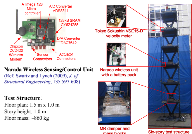
Fig. 2: Experimental Setup
