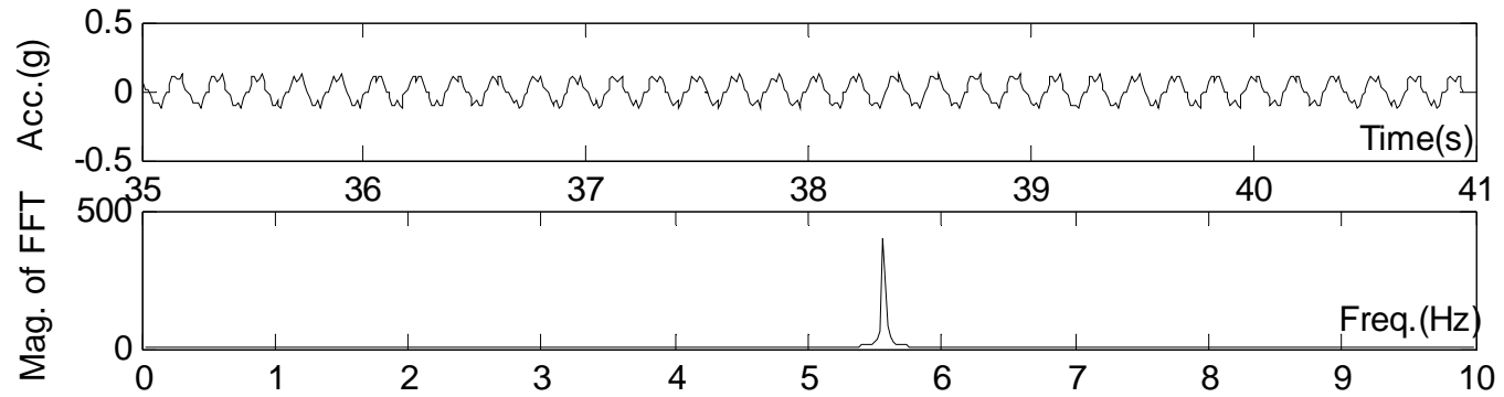
(a) Harmonic ground motion acceleration
