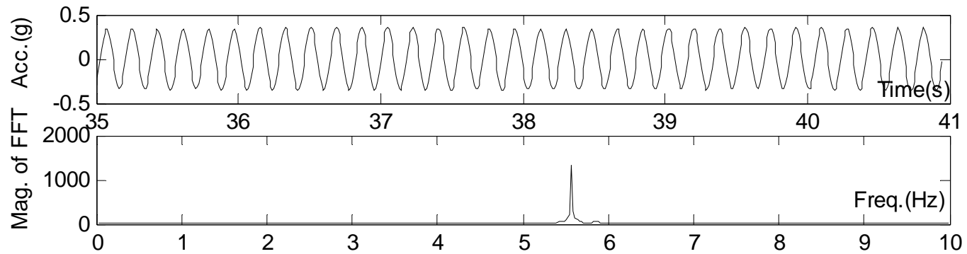
(b) Acceleration response of the third floor
