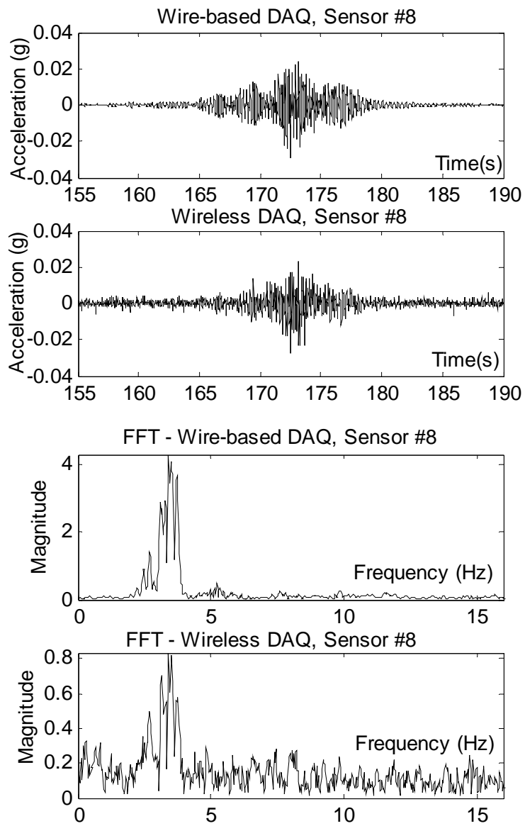
(a) Time-history responses and FFT results for sensor location #8
