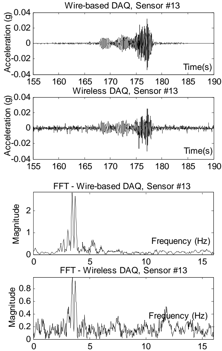
(b) Time-history responses and the FFT results for sensor location #13
