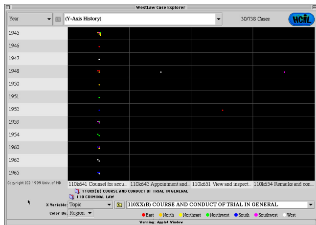
Figure 4b: GRIDL showing legal information after two category expansions on the x-axis, 110 Criminal Law and 110XX(B) Course and Conduct of Trial in General
