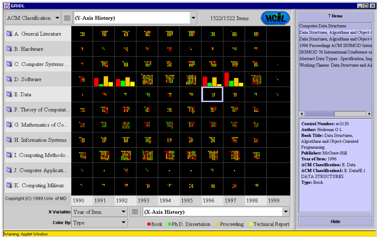
Figure 4c: GRIDL with the ACM Computing Classification System, after user clicks on a cluster
