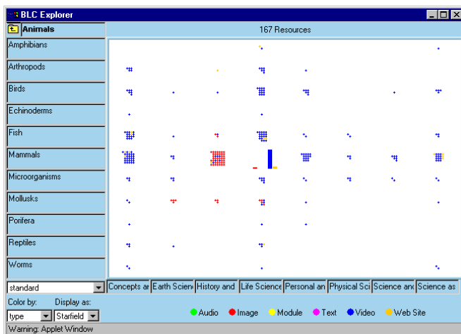
Figure 2: Expanding the “Animals” Category on the y-axis in the early version of GRIDL
